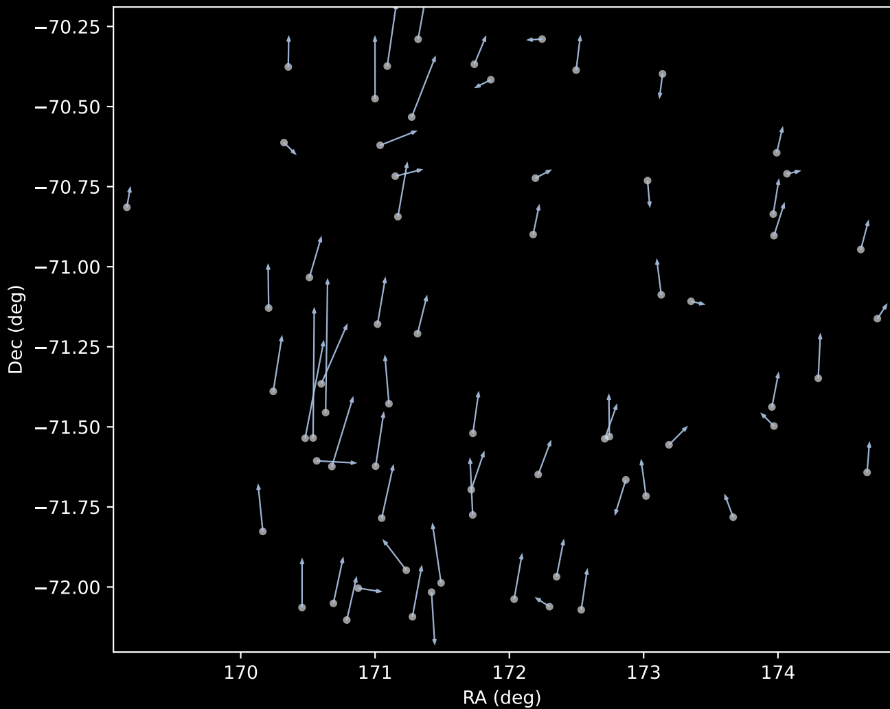
GALAH DR4 Cluster 1 Proper Motion Vectors (n=67)
