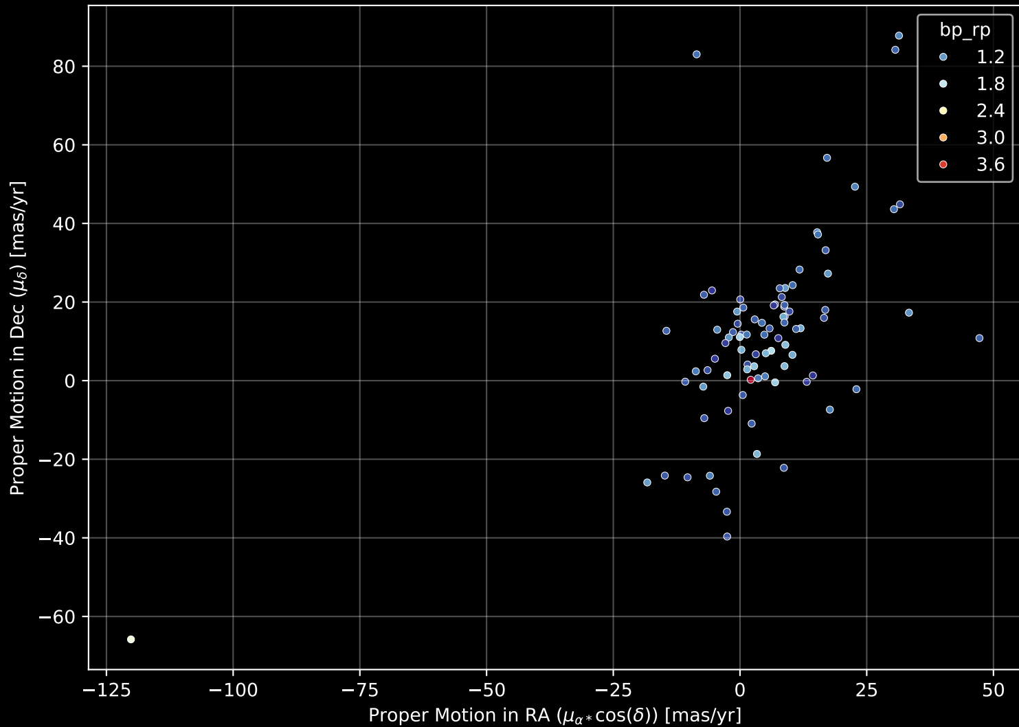
GALAH DR4 Field: [7176] Proper Motion Diagram (n= 87)
