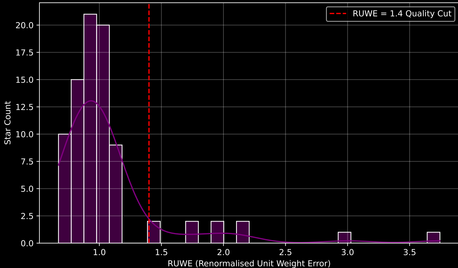
GALAH DR4 Field [7176] RUWE Distribution (n= 85)
