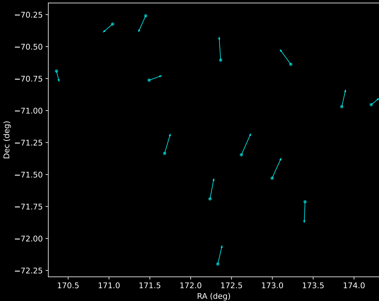
GALAH DR4 Noise Stream Proper Motion Vectors (n=14)
