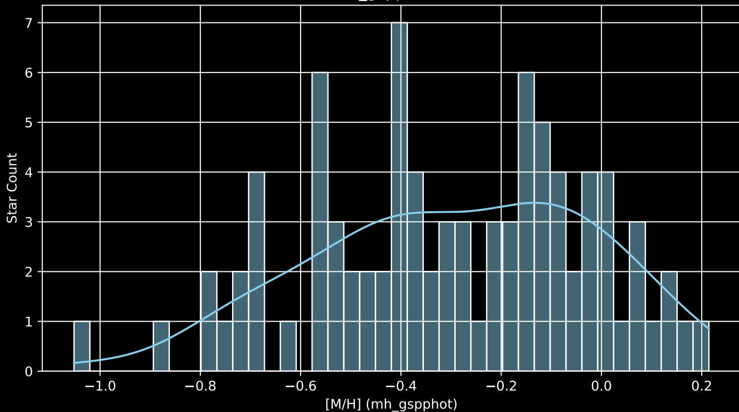
GALAH DR4 Field: [7176] [M/H] (mh_gspphot) (n= 87)
