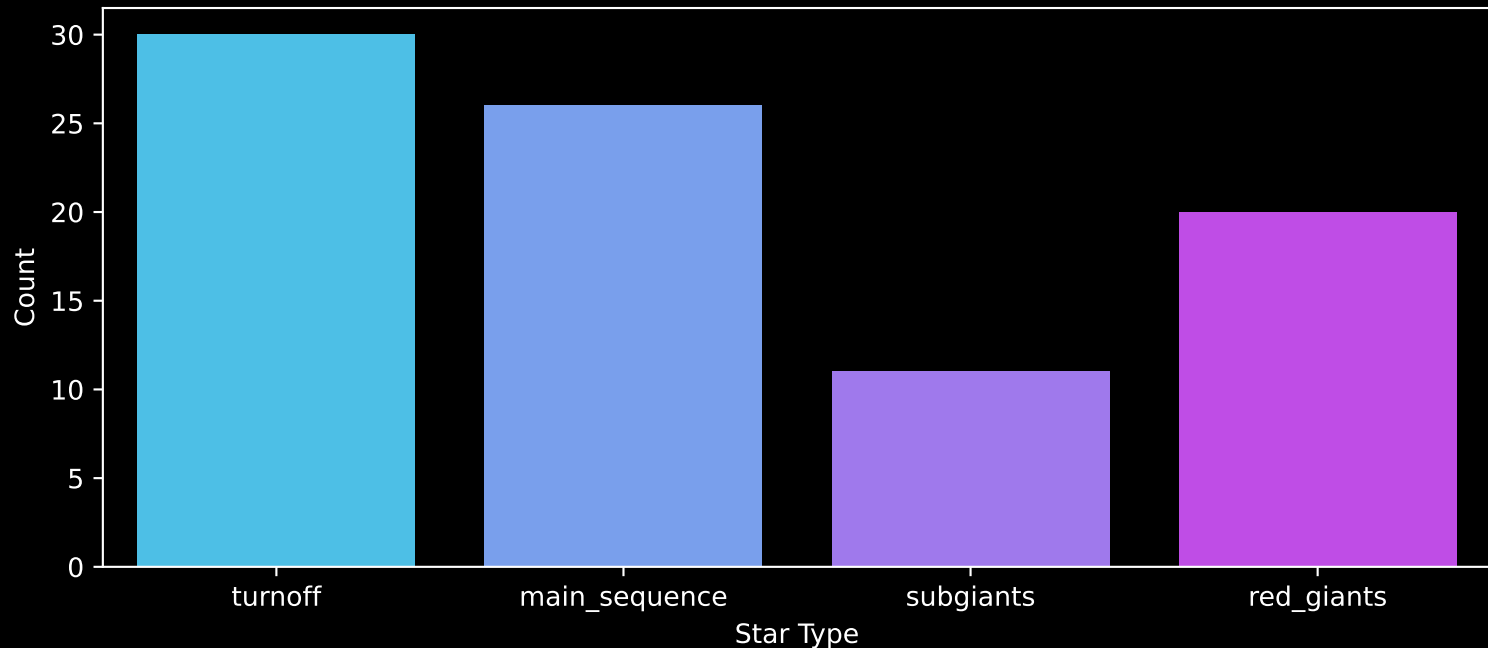
GALAH DR4 Field: [7176] Count plot of Star Type
