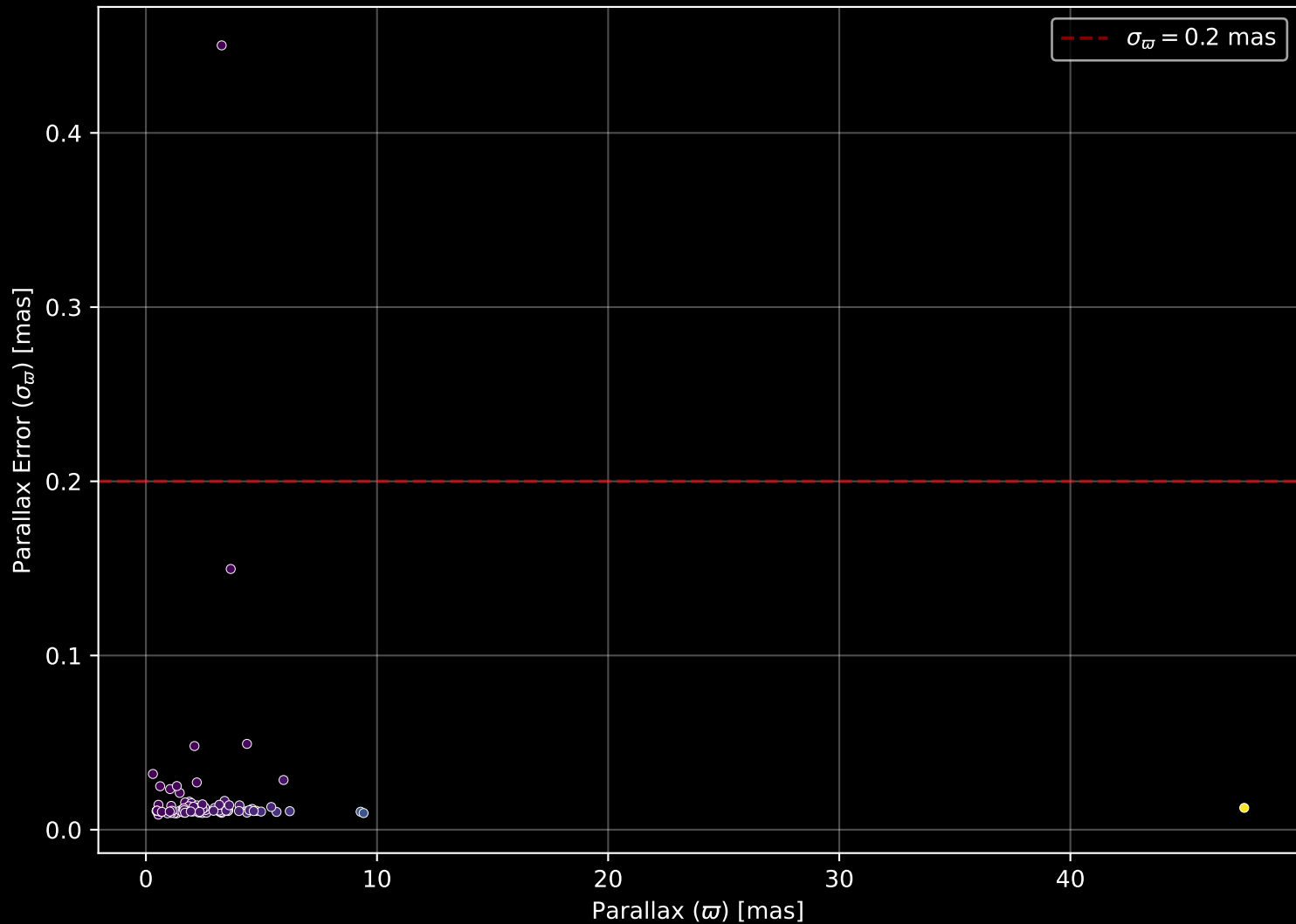
GALAH DR4 Field: [7176] Parallax Quality (n= 87)
